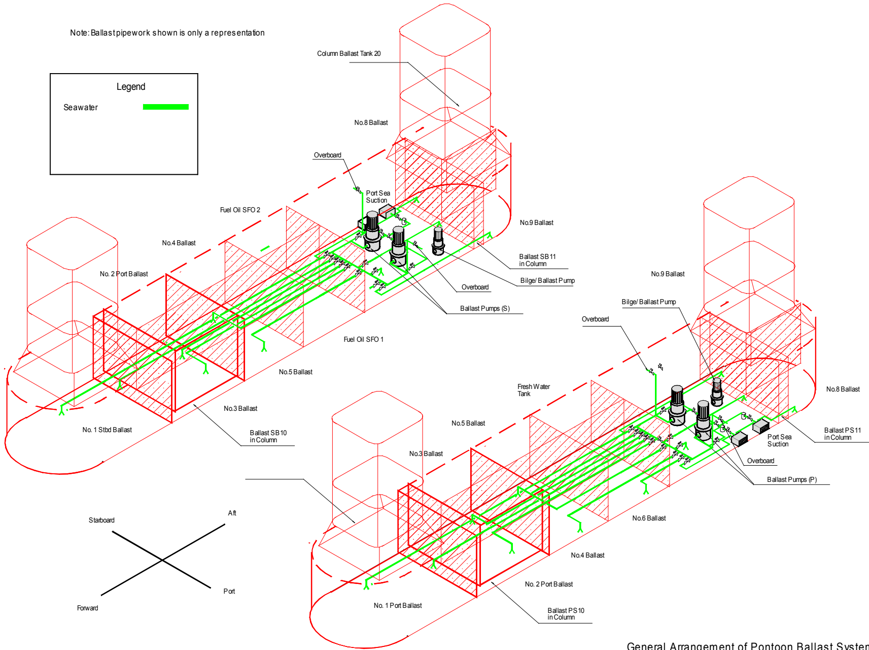
General Arrangement of Pontoon Ballast System
